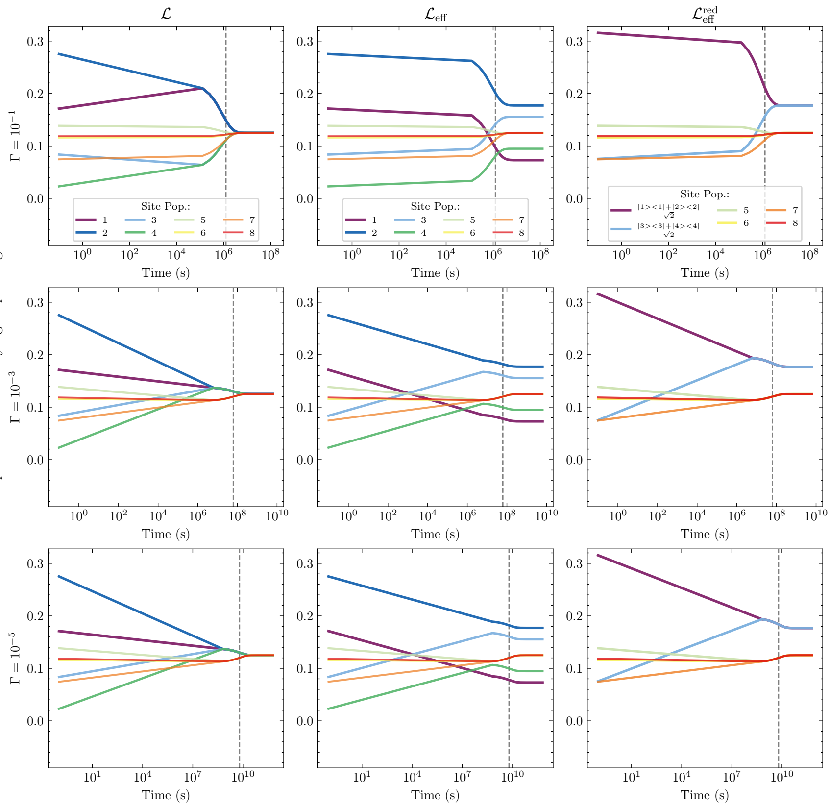
Time Evolution of Site Populations under \mathcal{L} , \mathcal{L}_{\text{eff}} , and \mathcal{L}_{\text{eff}}^{\text{red}} N=8 ; N_{\text{dimers}}=2 ; N_{\epsilon}=4 ; J = 10^{-1} ; \epsilon = 10^{-4} ; seed=680
